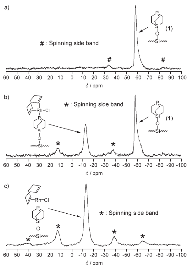
Figure 1. a) ^{31}\text{P} CP/MAS NMR spectrum of 1 ; b) ^{31}\text{P} CP/MAS NMR spectrum that was obtained from 1 and a substoichiometric amount of [\text{RhCl}(\text{cod})]_2 (P/Rh 1:0.48); c) ^{31}\text{P} CP/MAS NMR spectrum that was obtained by treating 1 with excess [\text{RhCl}(\text{cod})]_2 (P/Rh 1:1.52) before washing and drying.
